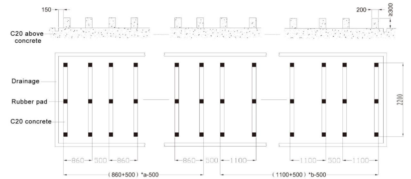
b. Concrete foundation diagram
