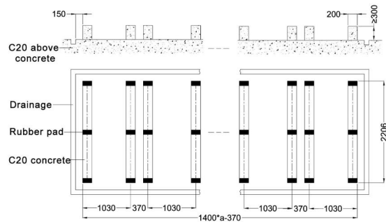
b. Concrete foundation diagram
