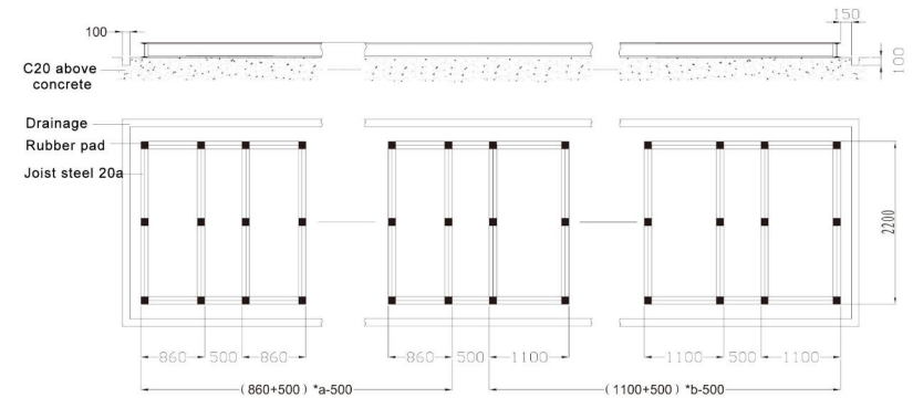
a. Joist steel foundation diagram
