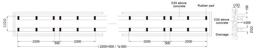
b. Concrete foundation diagram
