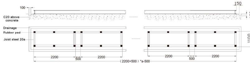
a. Joist steel foundation diagram
