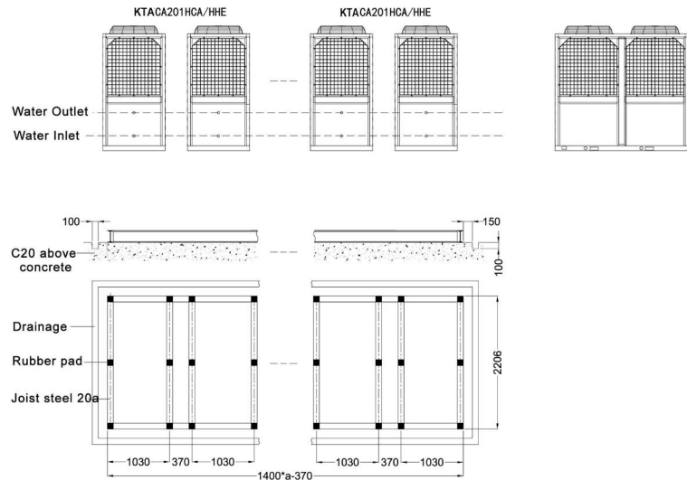
a. Joist steel foundation diagram
