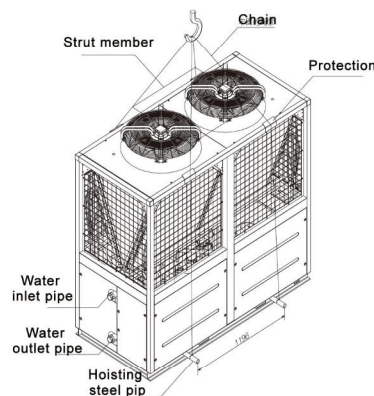
Example lifting schematic for TCA201
