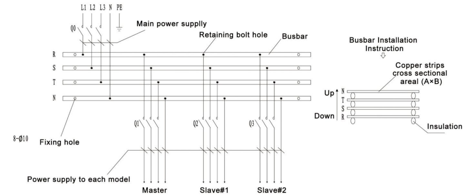
Example lifting schematic for TCA203
