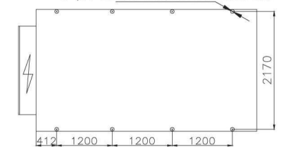
Base vibration absorption installation diagram 8-φ14 vibration absorption installation hole
