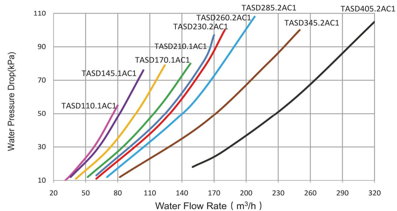
Air-Cooled Screw Water Side Exchanger Water Pressure Drop Diagram
